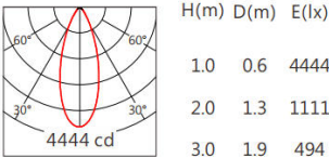
JR-5050 40° 3000K
