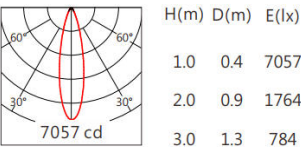
JR-5050 30° 4000K
