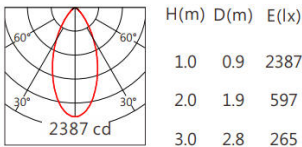
JR-5050 55° 4000K
