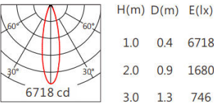
JR-5050 30° 3000K
