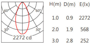
JR-5050 55° 3000K
