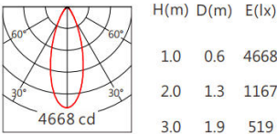
JR-5050 40° 4000K
